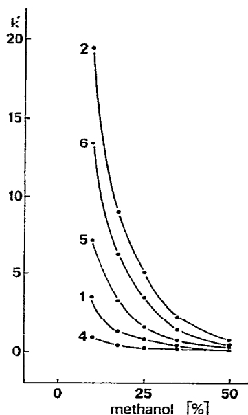
Fig. 2. Influence of methanol concentration on column capacity ratios. Mobile phase: 10 mM tributylammonium formate (pH 3.0). Solute (see Table I): 1 = cAMP; 2 = N 6 -monobutyril-cAMP; 4 = 8-amino-cAMP; 5 = 8-dimethylamino-cAMP; 6 = 8-benzylamino-cAMP.
